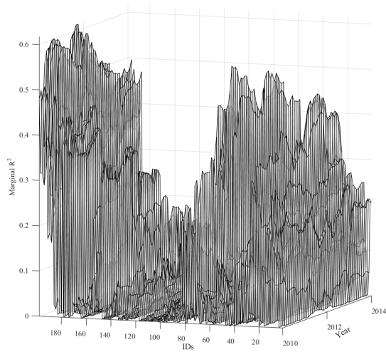
(a) \Delta \hat{F}_1 from the Rolling Window Scheme
