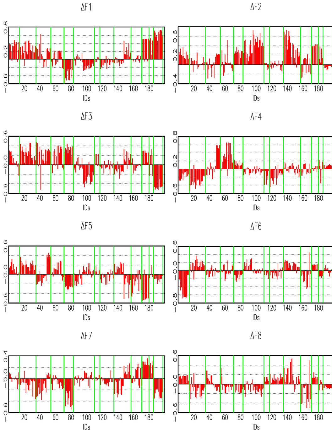
Figure A3. Factor Loading Coefficients Estimates
