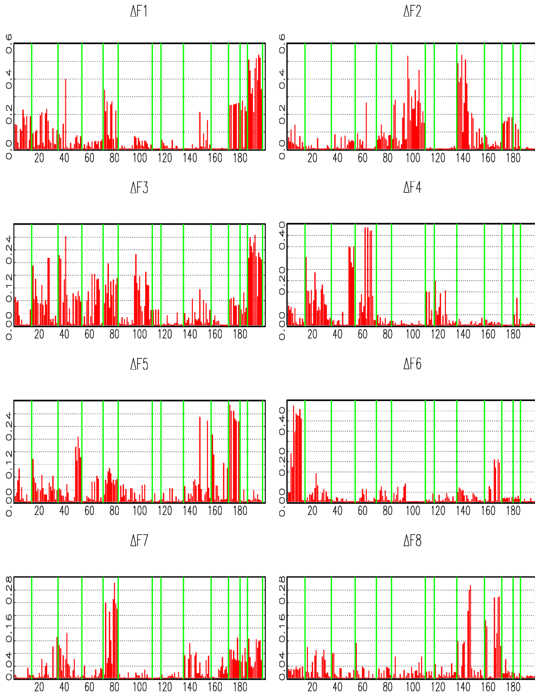
Figure A4. Marginal R^2 Analysis
